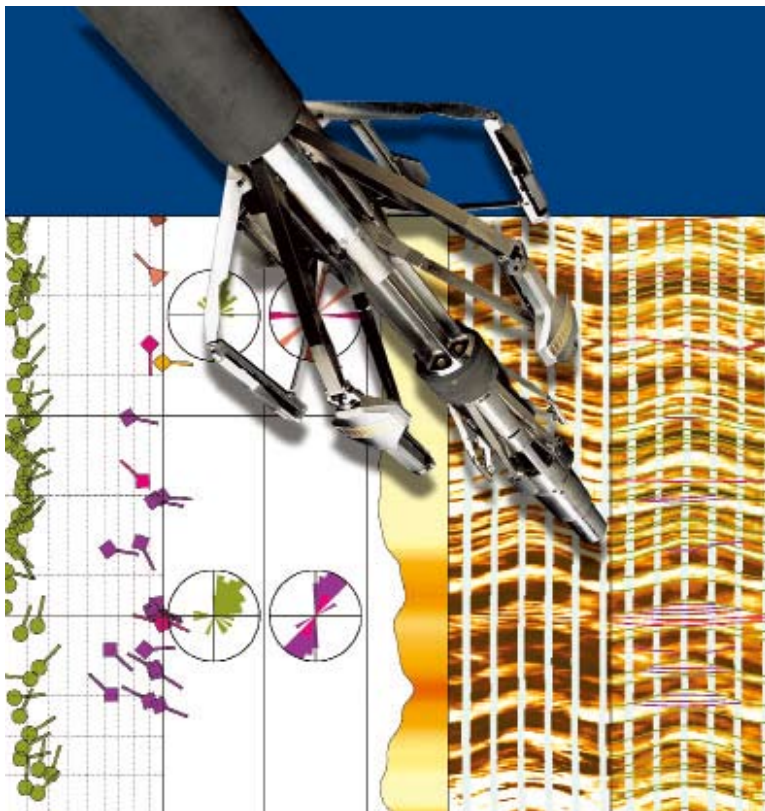
Example of EARTH Imager high-resolution resistivity images illustrating bedding and fracture dip magnitudes and orientations.
